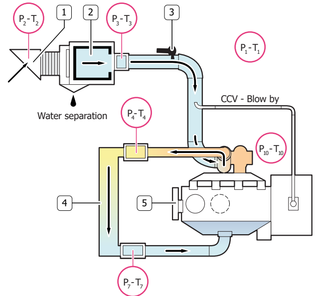
Figure 4. Generic Air Intake System layout
