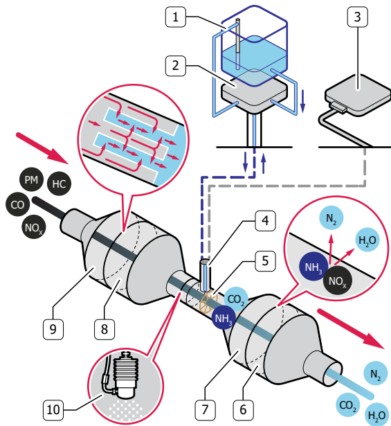
Figure 3. HI-eSCR - T4B and Euro VI
